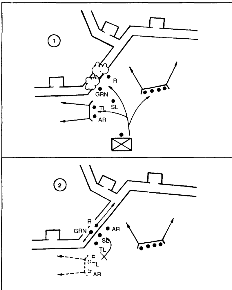
Figure 4-11. Enter a trench (squad).
